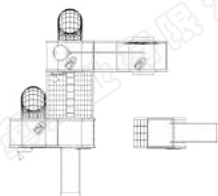
平面图 规格: 12.2m*7.1m*3.7m
